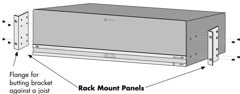
Figure 1: Fastening the Rack Mount Panels.
